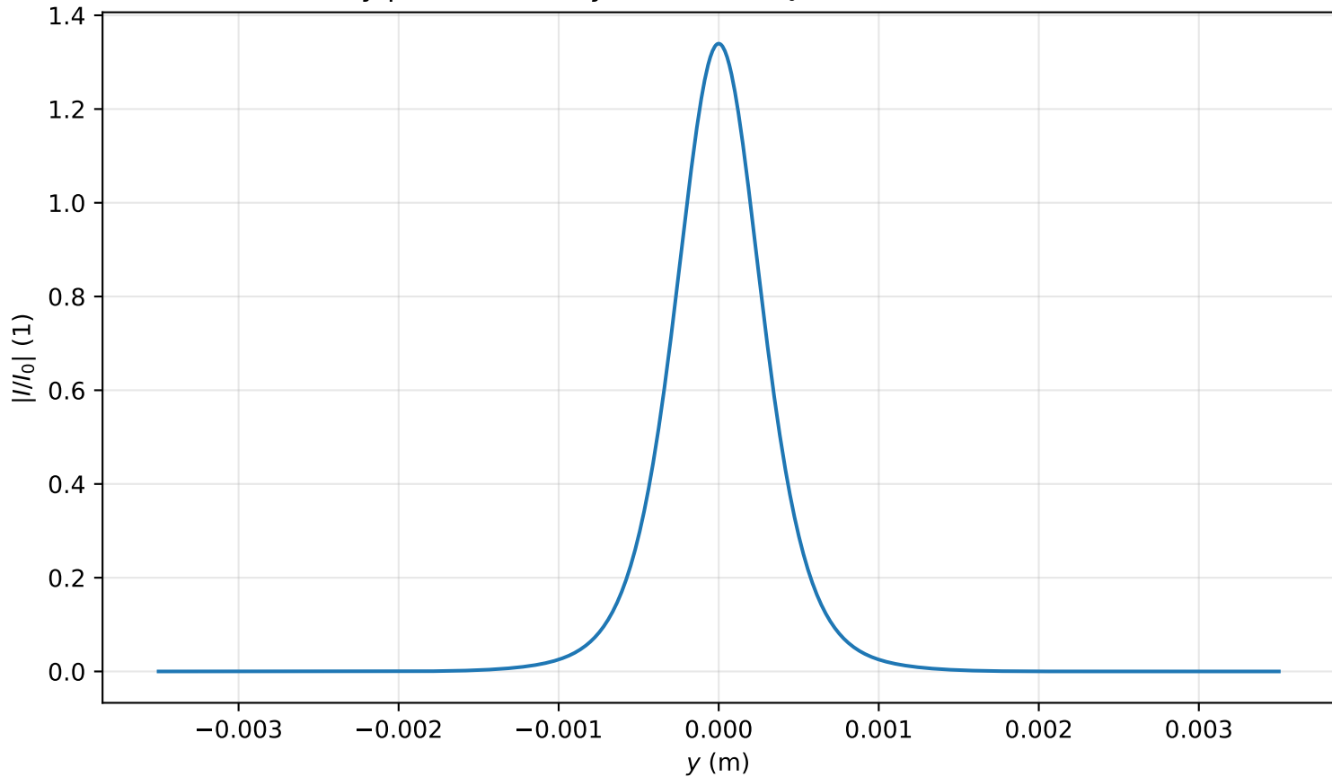
Intensity profile I(x=0, y, z=1.831)/I_0 , P_{in}=0.8P_{cr} , artificial time
